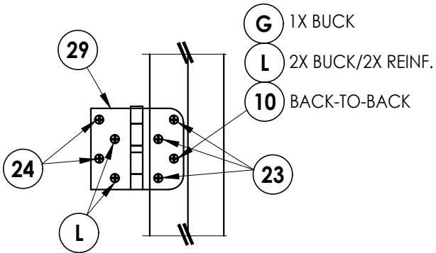
HINGE DETAIL
