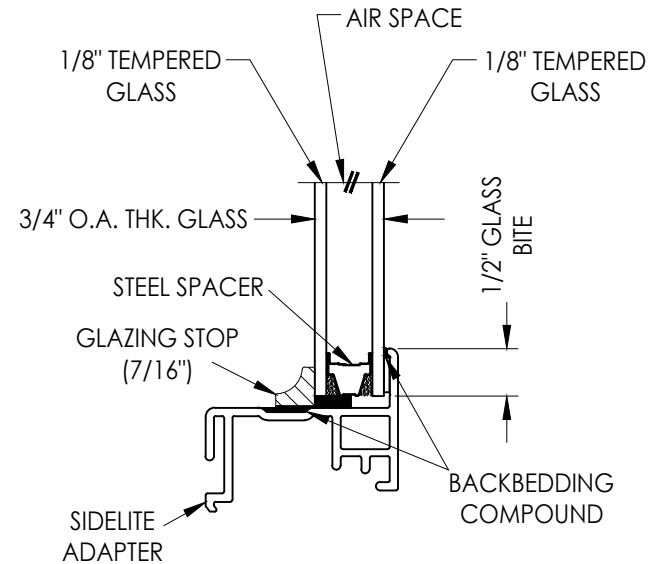
G4 GLAZING DETAIL 3/4" Insulated Glass
